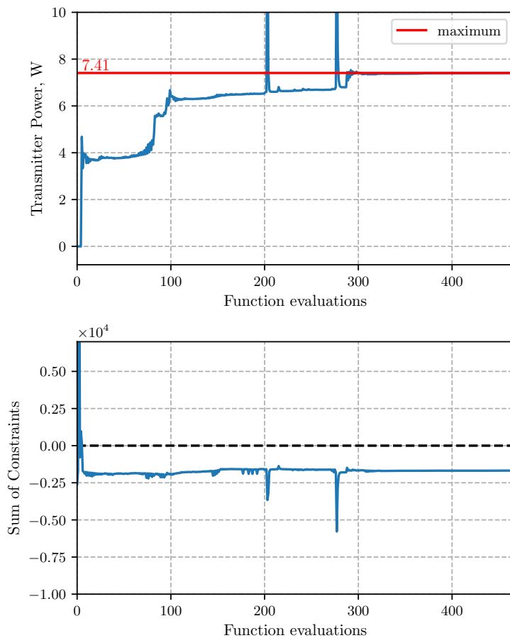
Fig. C.2. Optimization convergence history of MS uncoupled model. Total run time on Intel Core i5-5300U processor: 5530 s.
