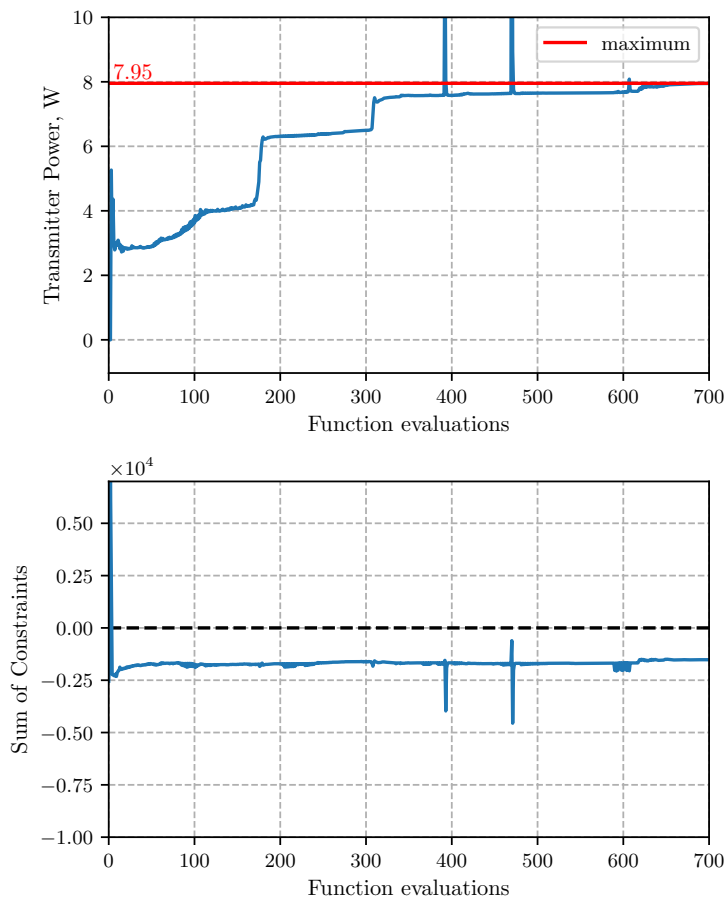
Fig. C.1. Optimization convergence history of MS coupled model. Total run time on Intel Core i5-5300U processor: 9336 s.
