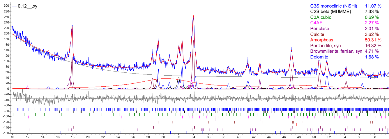
Fig. C.4. Quantitative Rietveld phase analysis for cement paste modified by 0.12 % bwoc of MWCNT
