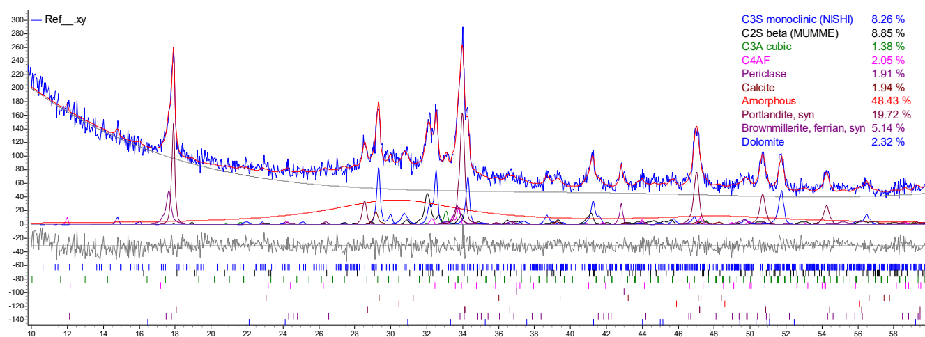
Fig. C.1. Quantitative Rietveld phase analysis for cement paste without admixtures (reference)
