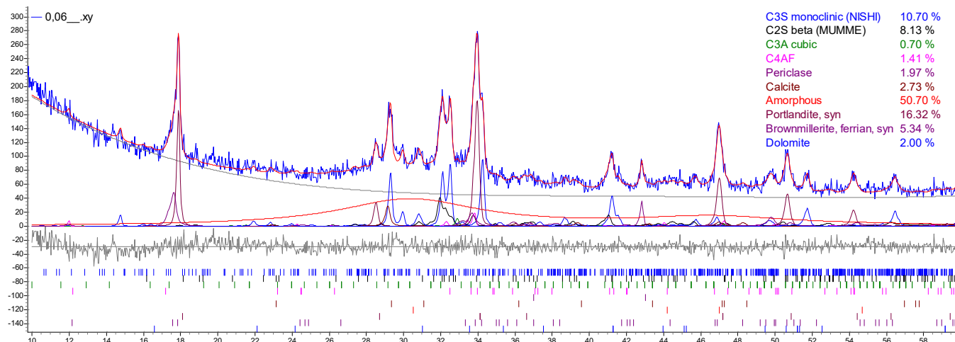
Fig. C.2. Quantitative Rietveld phase analysis for cement paste modified by 0.03 % bwoc of MWCNT
