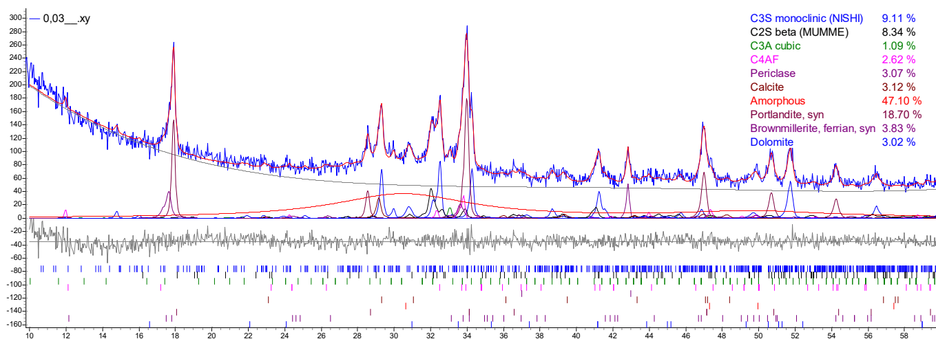
Fig. C.2. Quantitative Rietveld phase analysis for cement paste modified by 0.03 % bwoc of MWCNT
