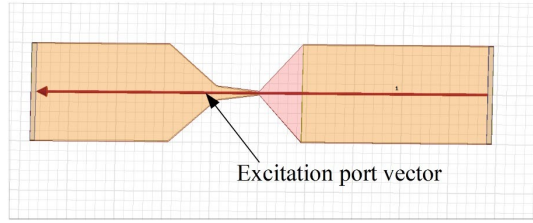
Fig. 4.4. View of the excitation port for the electric field in the model
