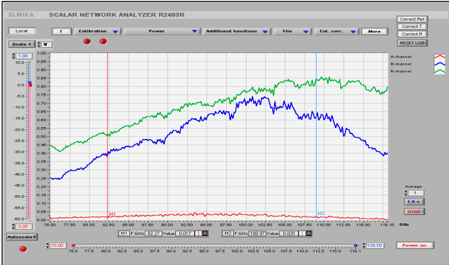
Fig. 2.30. Virtual control panel for the detected voltage on the frequency and on power measurement setups in W- and D-bands using a waveguide detector mount
