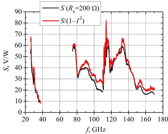
Fig. 2.34. Voltage sensitivity on the frequency of the MW diode having the zero-bias voltage electrical resistance R_0 = 200 \text{ }\Omega with the evaluation of power losses due to reflectance in the measurement system S/(1-I^2) and without it, S
