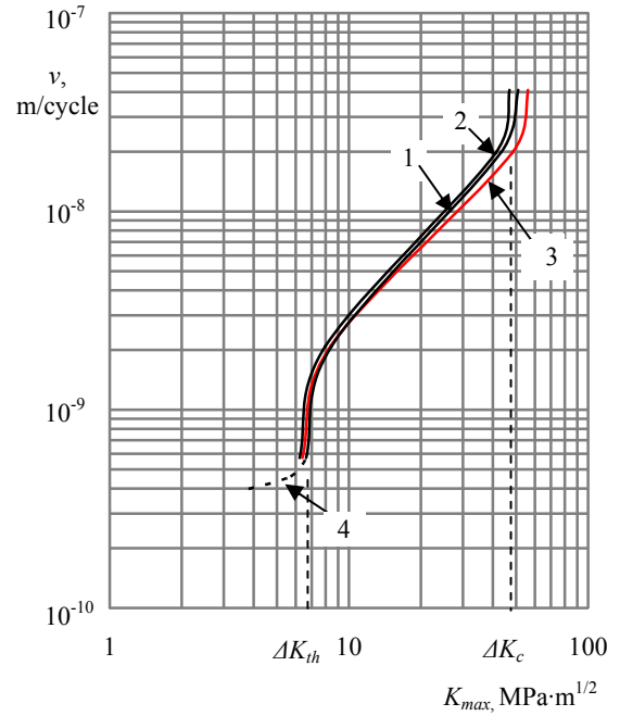
Fig. 5 Kinetic diagram of fatigue: 1 - Anderson, 2 - Tada, Paris, Irvine, 3 - ASTM, 4 - short crack
